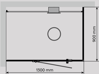
VISTA 130 RIGHT Size: D 900 x W 1 300 mm
