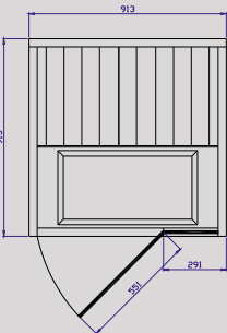
TYLÖSAND T-810 Size: D 913 x W 913 mm Power: 1350 W
