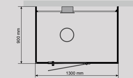
VISTA DCO 130 LEFT Size: D 900 x W 1 300 mm
