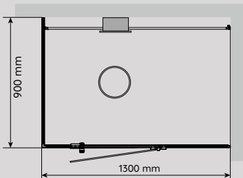
VISTA 130 LEFT Size: D 900 x W 1 300 mm
